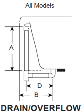
DRAIN/OVERFLOW
