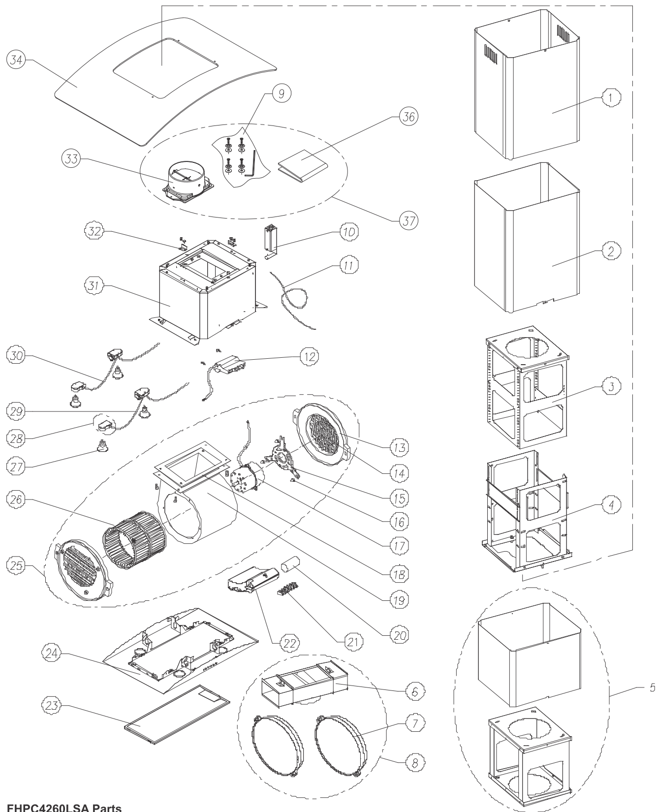
FHPC4260LSA Parts
