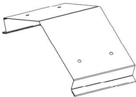
A4M01127 RIDGE CAP SPLICE (x2)
