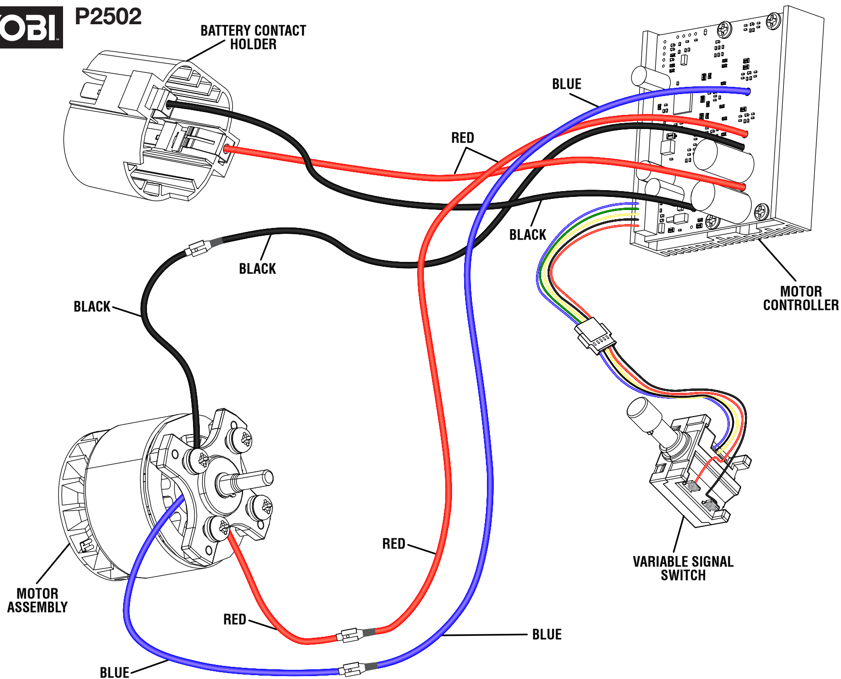
WIRING DIAGRAM
