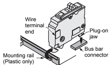
Figure 5: QO Tandem Circuit Breaker
