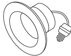
NICOR-Downlight Model # DLR56-3008-120-4k-XX 12.00W (4000K)
