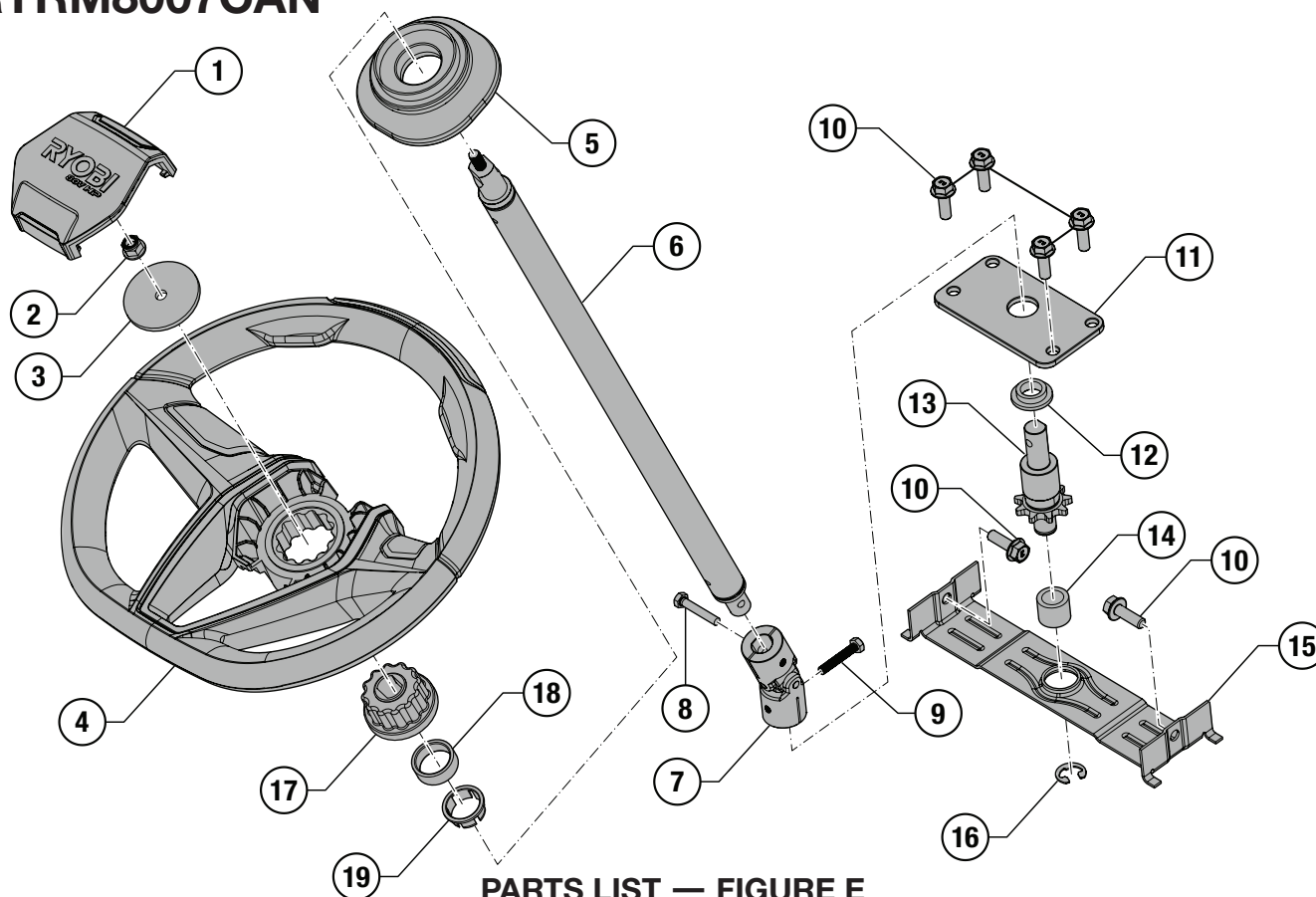
FIGURE E — STEERING COLUMN ASSEMBLY
