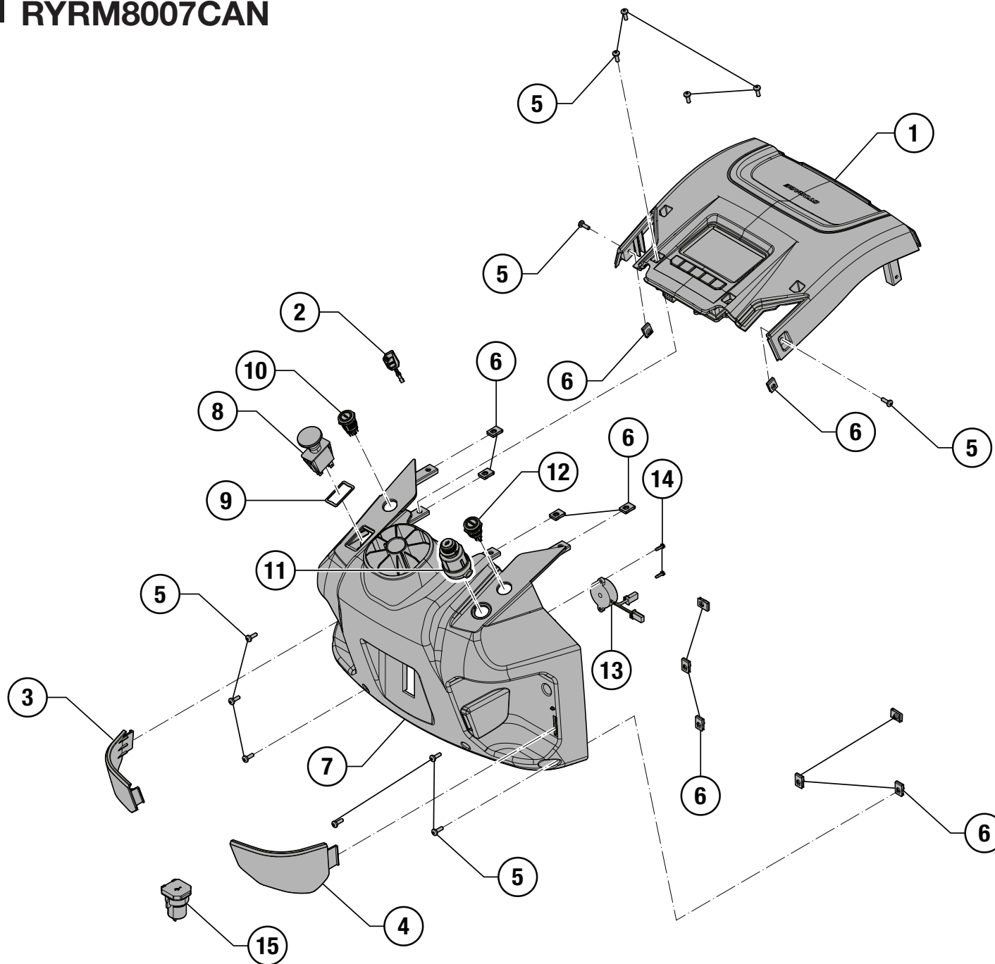
FIGURE M — CONTROL PANEL ASSEMBLY
