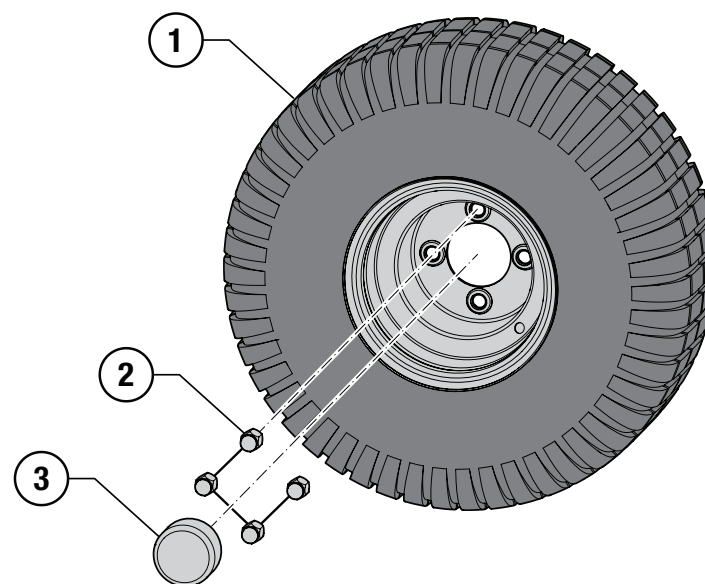
FIGURE A — WHEELS AND HUB COVERS
