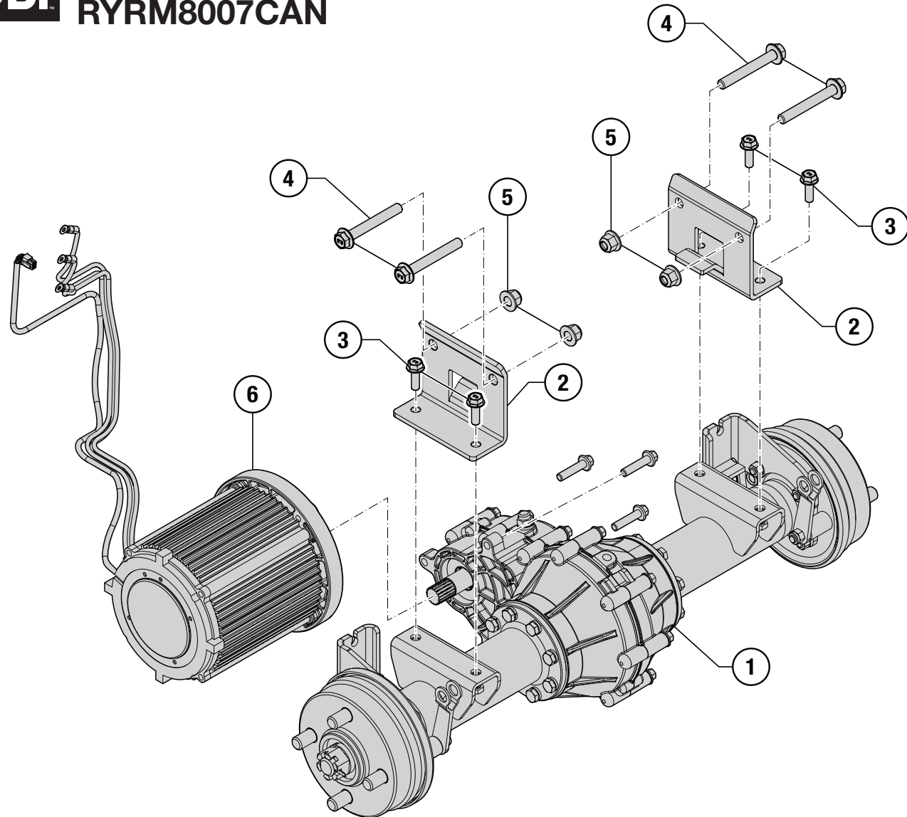
PARTS LIST — FIGURE I
