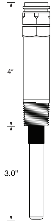
48-226 Standard 1/2" NPT OMSID# 317904087
