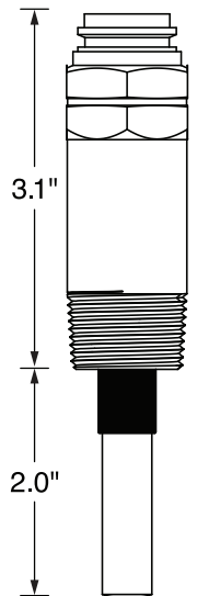
48-204 Extended 3/4" NPT Short Insertion OMSID# 317904095
