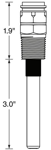
48-221 Standard 1/2" NPT OMSID# 317904089
