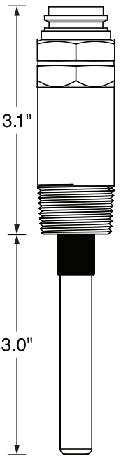
48-202 Extended 3/4" NPT OMSID# 317904085
