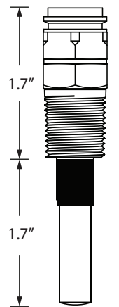
48-203 Standard 3/4" NPT OMSID# 317904093
