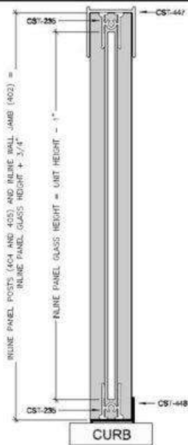
Legend Inline Panel vertical cross section
