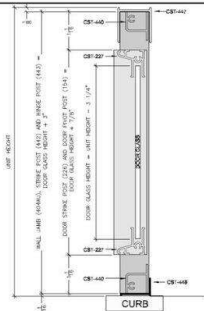
Legend Door vertical cross section
