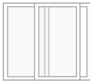
Sliding Window
