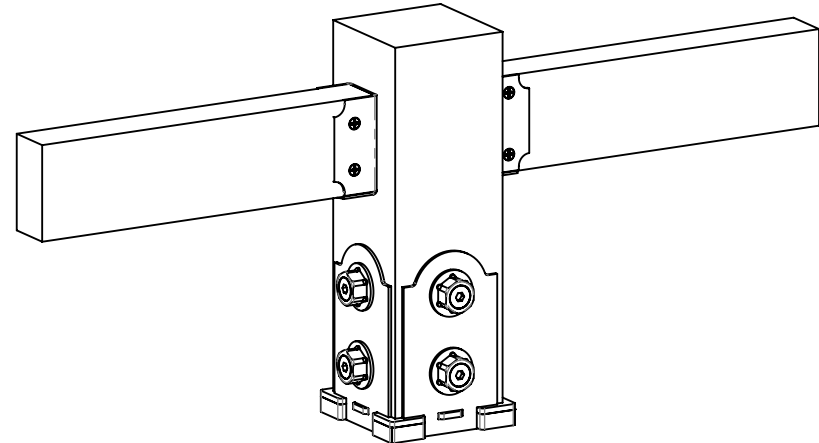
inline installation
