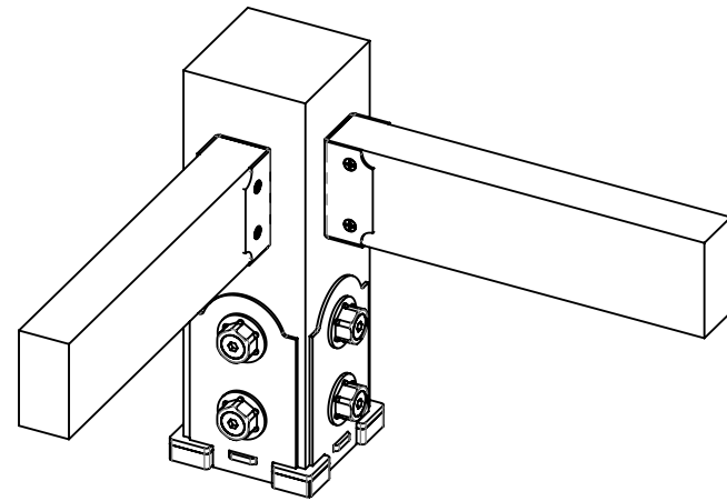
corner installation
