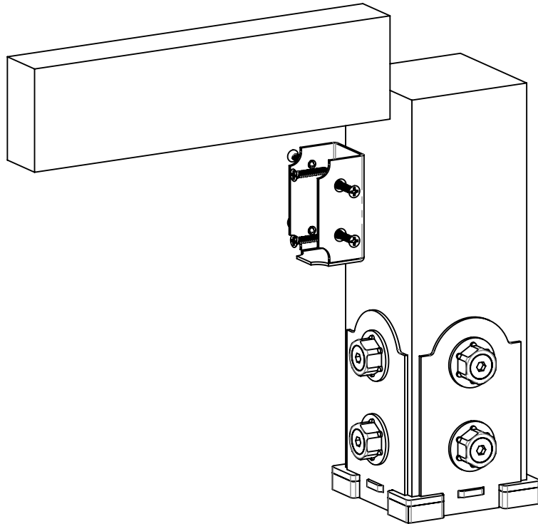
single rail installation (shown with 56607 Post Base)
