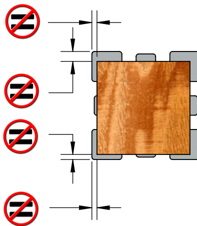
4x4 Post
