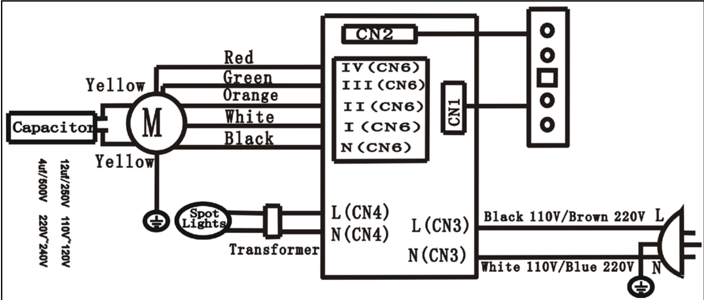
SV168/198 Series “R” Class Wiring Diagram
