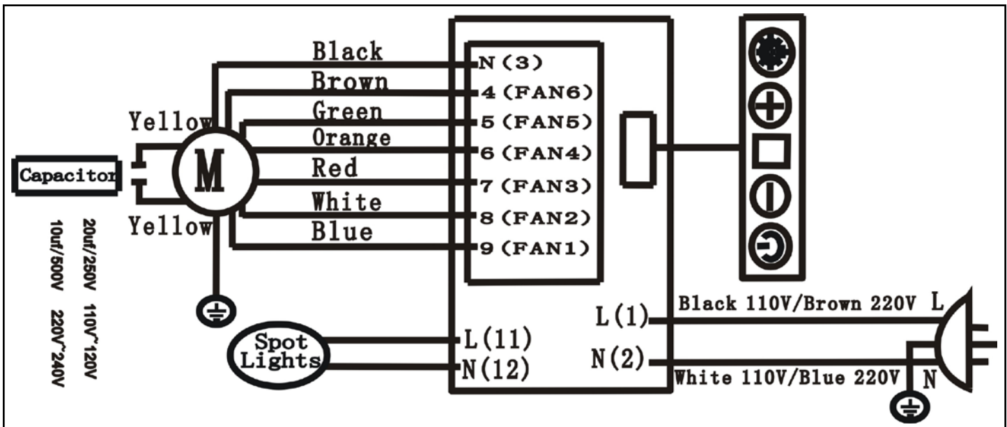
SV168/198 Series “E” Class Wiring Diagram (6 Speed)
