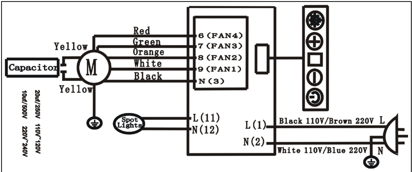
SV168/198 Series “E” Class Wiring Diagram (4 Speed)
