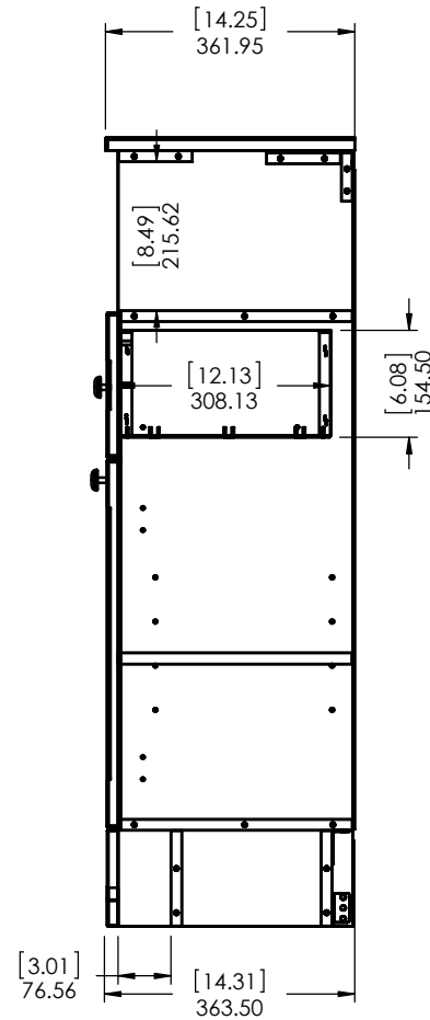
RIGHT VIEW
