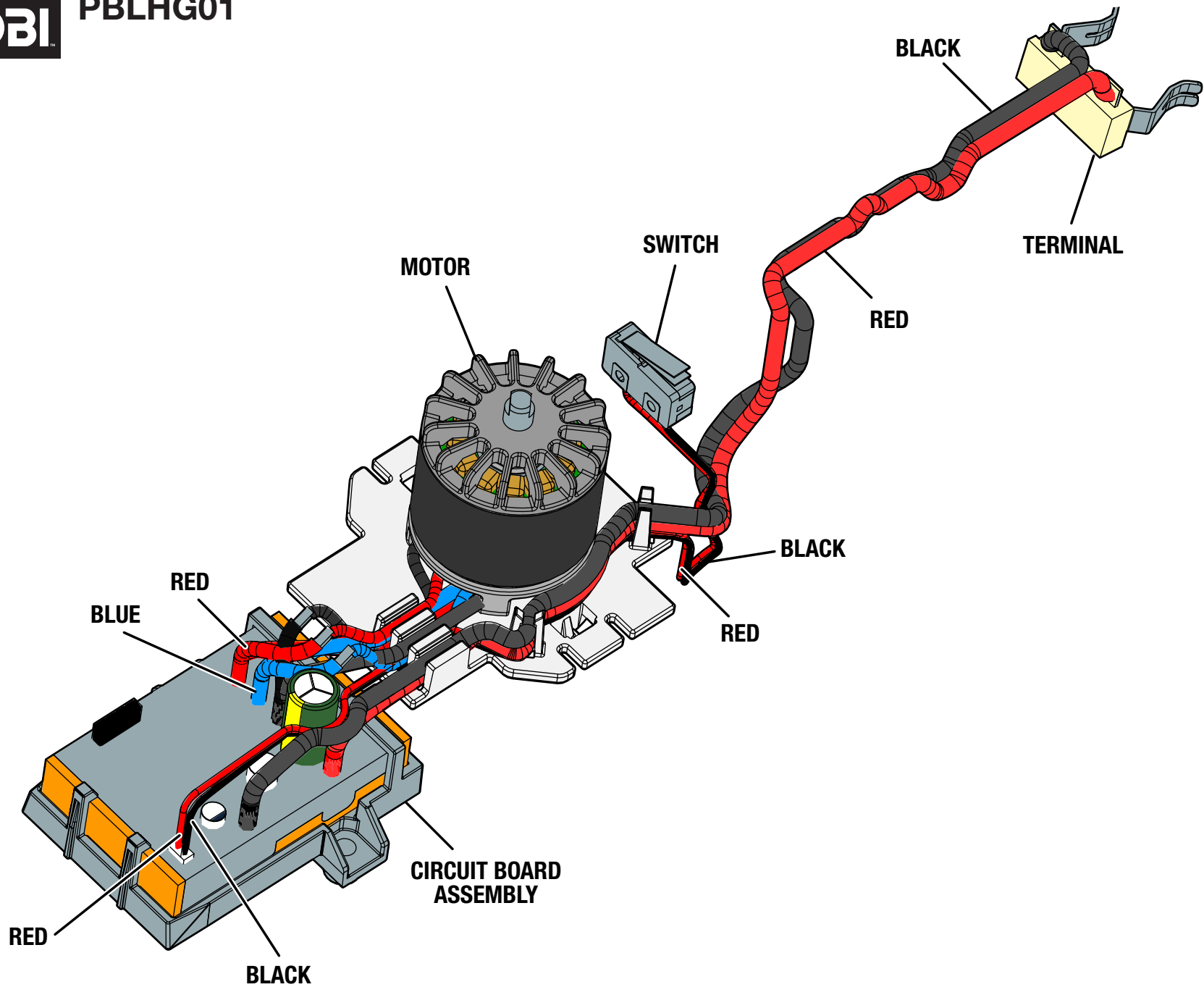
WIRING DIAGRAM
