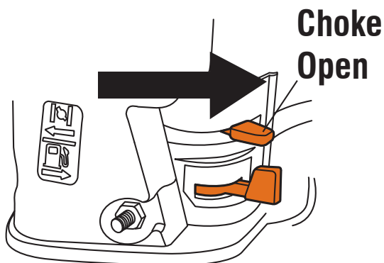
Figure 29 – Choke Lever
