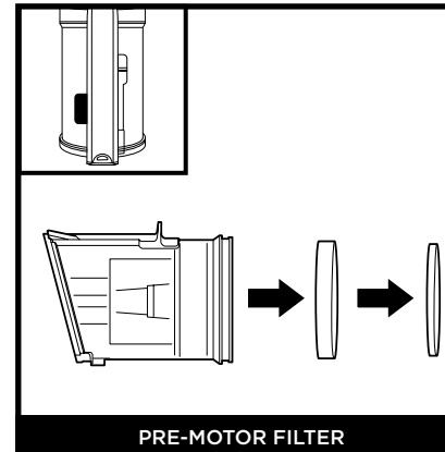
PRE-MOTOR FILTER
