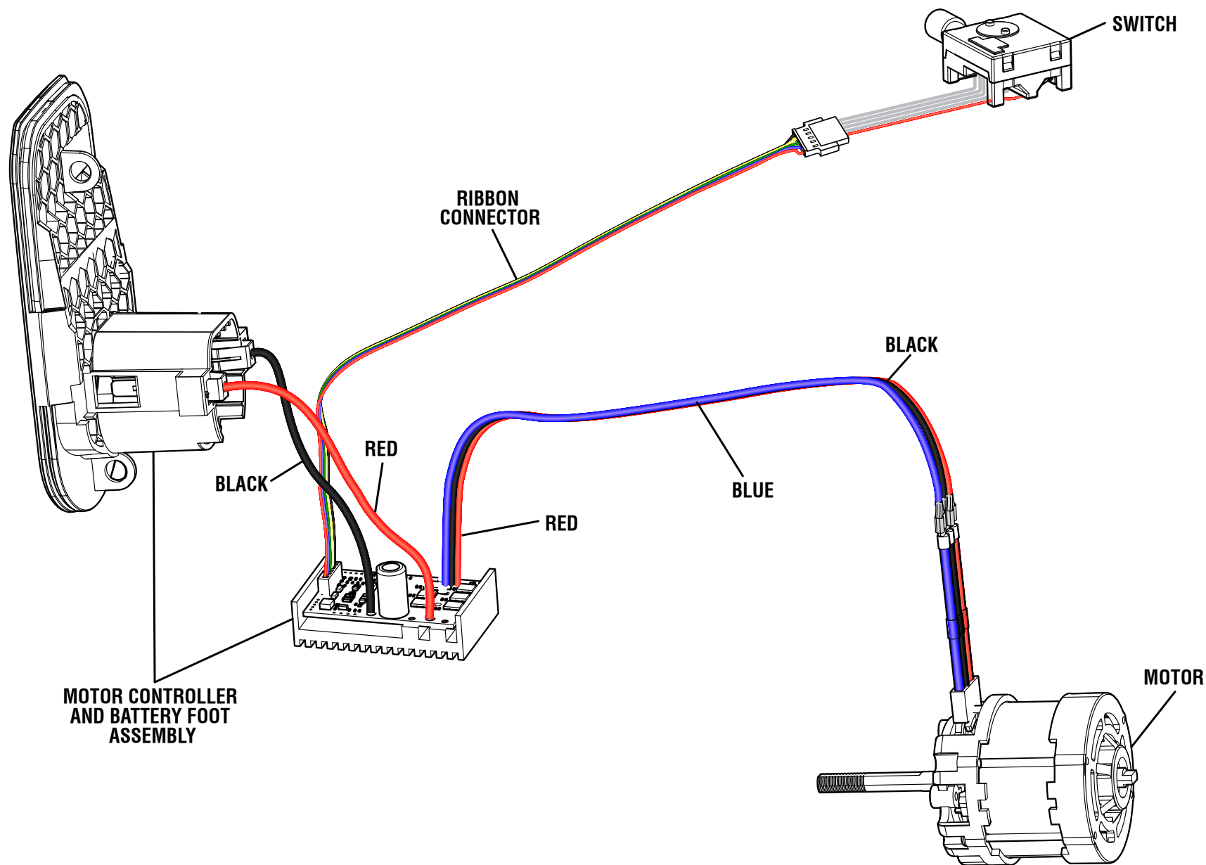
WIRING DIAGRAM
