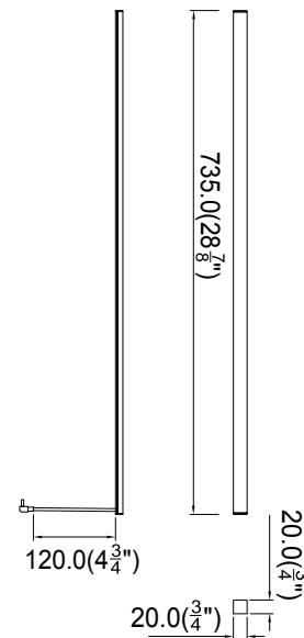
Light bar (optional) JS-BAR-30-001
