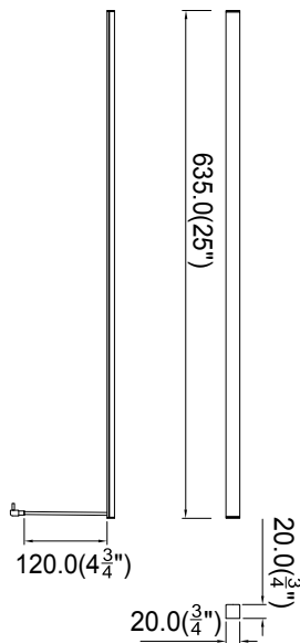
Light bar (optional) JS-BAR-26-001
