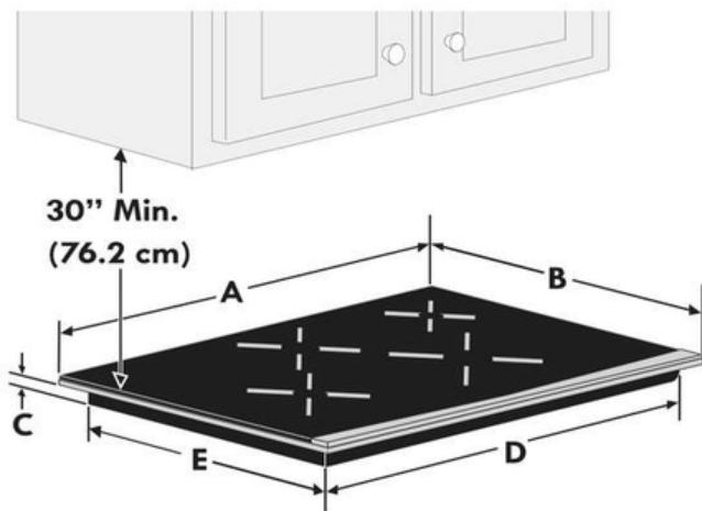
Cooktop Dimensions
