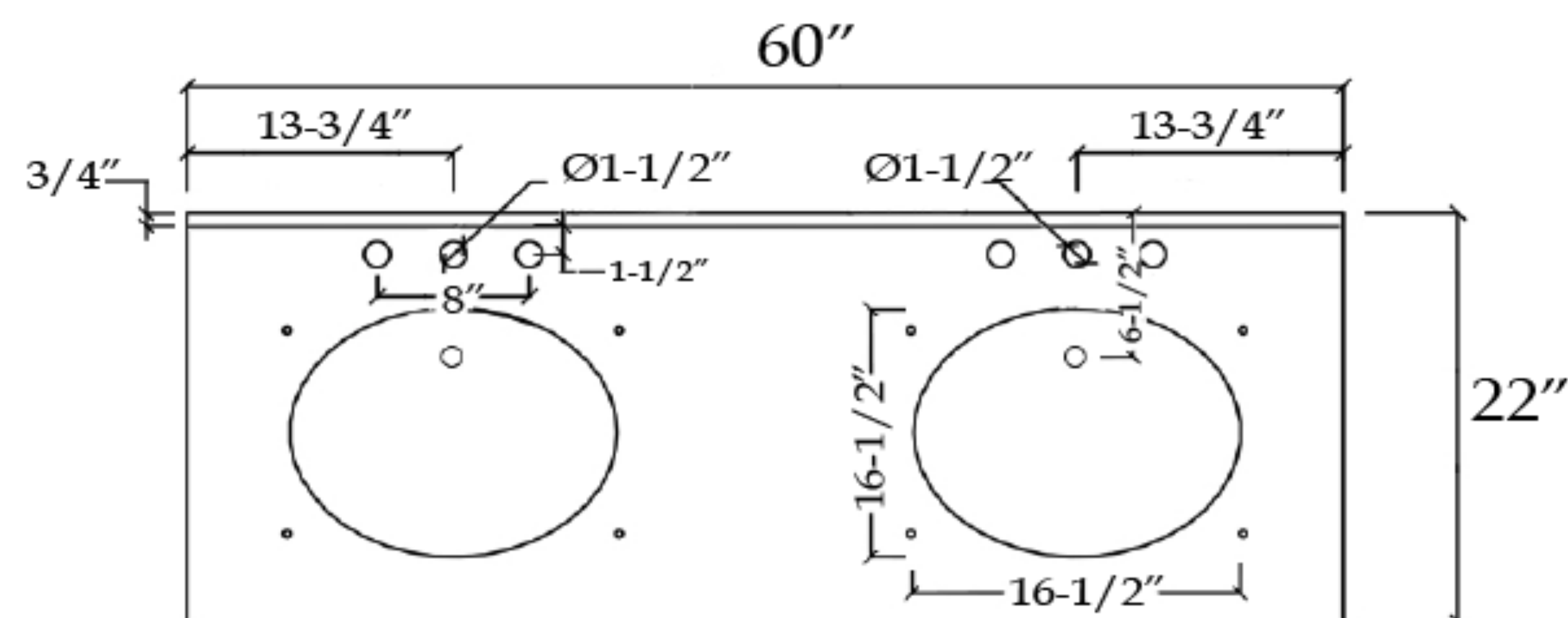
COUNTER-TOP
