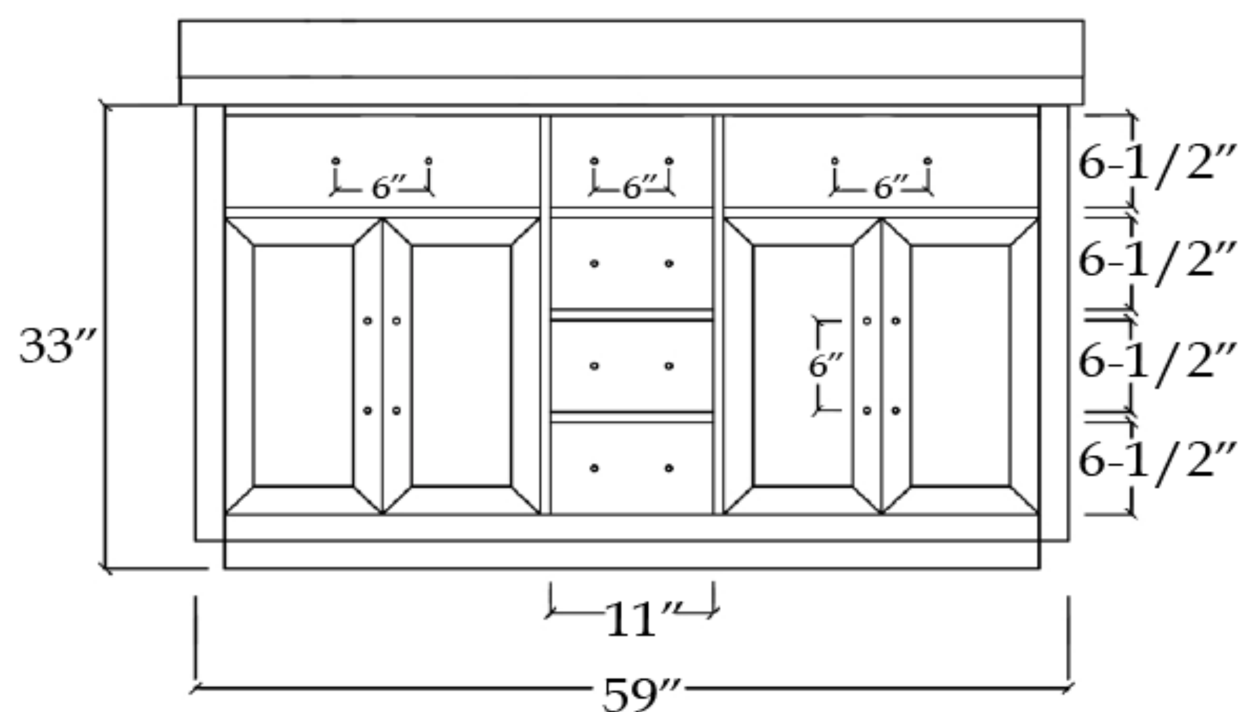
FRONT VIEW
