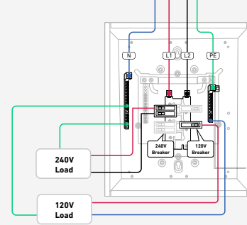
Ports of Home Power Panel and Transfer Switch
