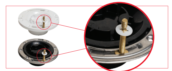
FAST SET™ STABILIZES BOLTS WITH BOLT SHELF™
