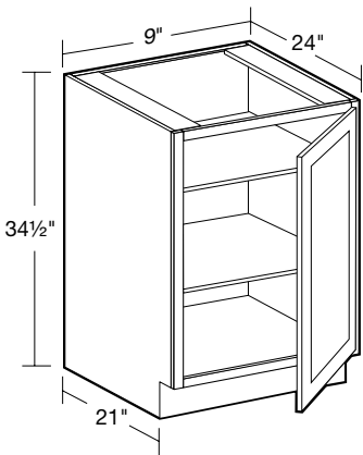
24" Deep Single Full Height Door
