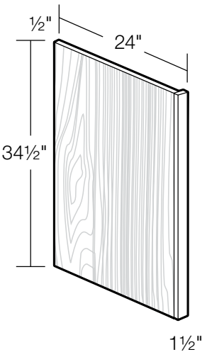
24" Deep End Panel with 1½" wide Filler
