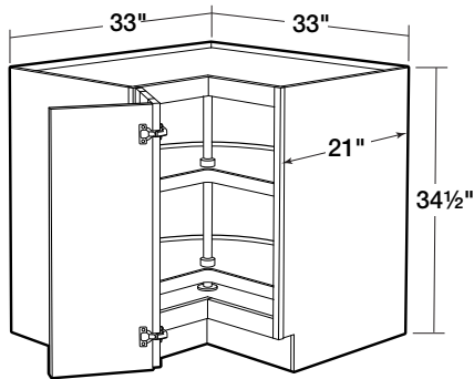
36" Easy Reach Super Suzan
