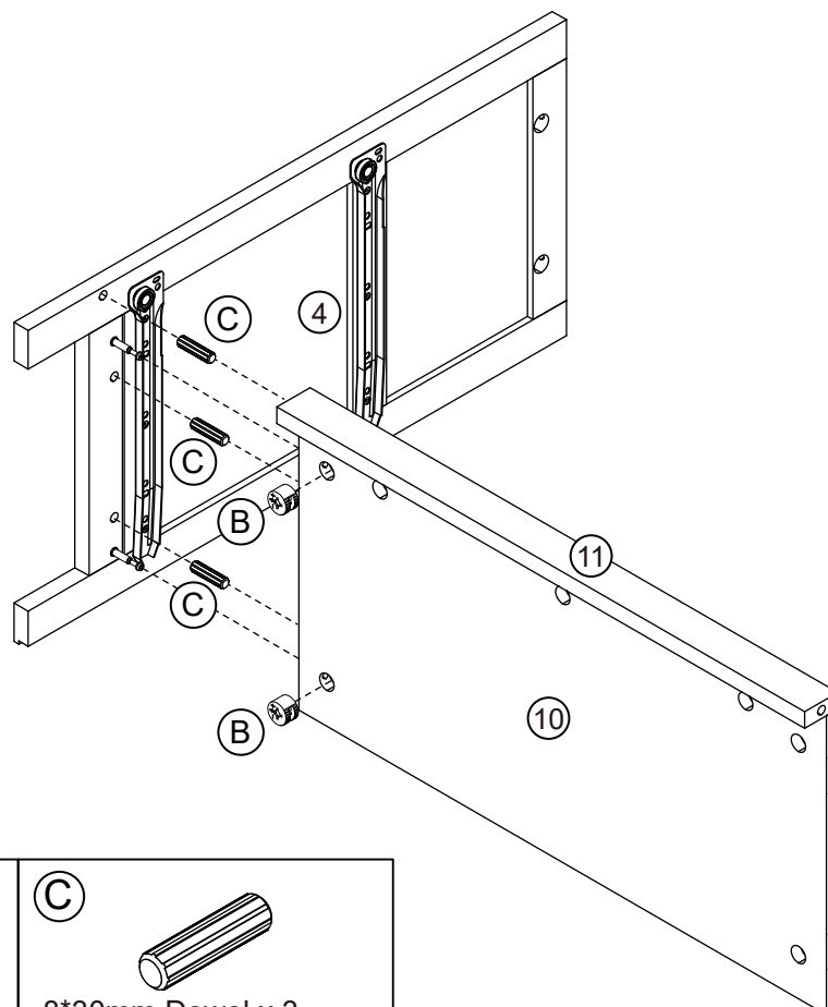
8*30mm Dowel x 3
