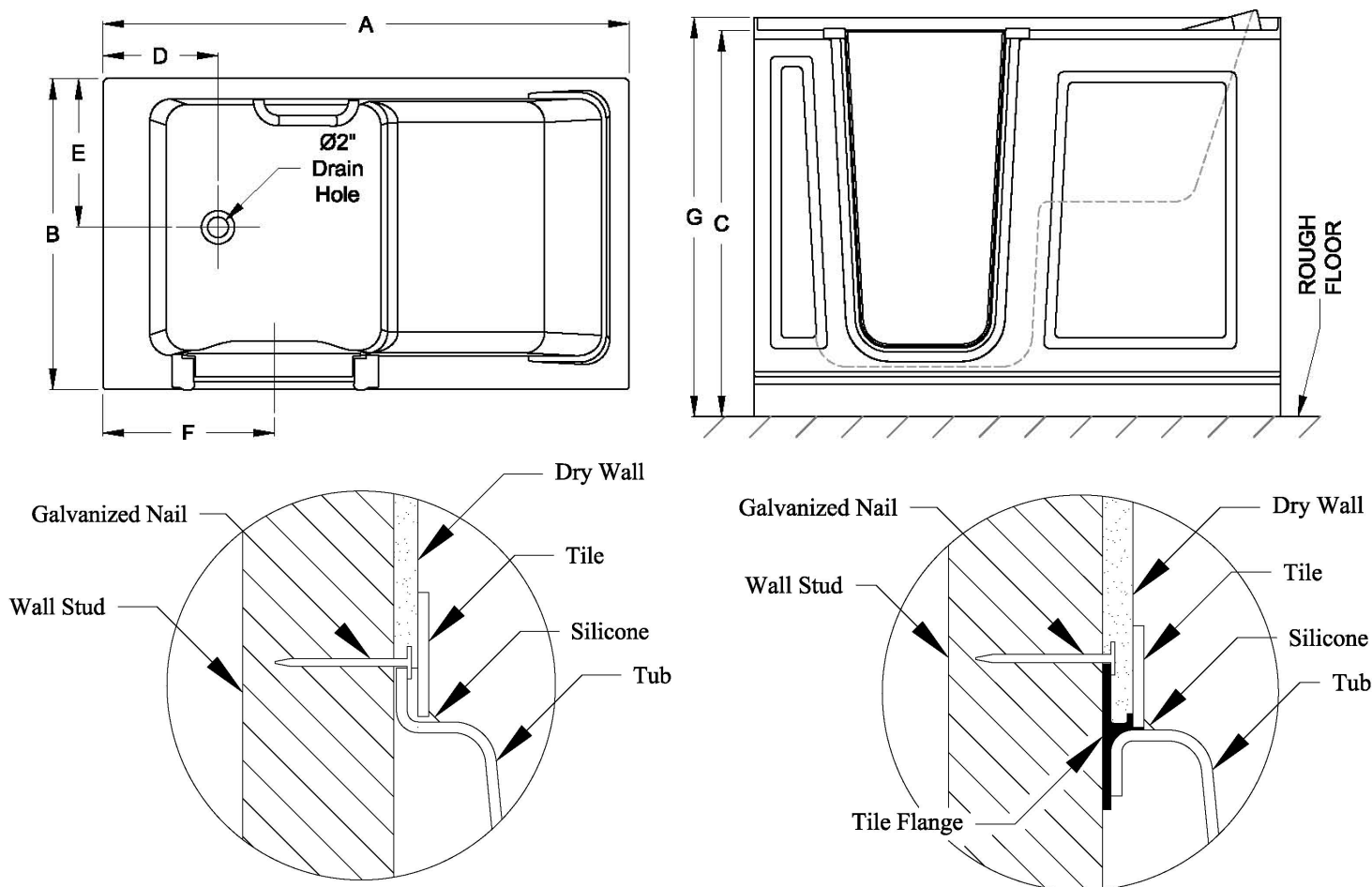
Integral Flange
