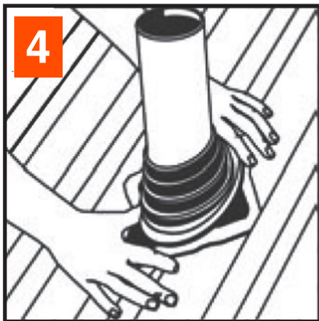
Form flashing base to roof profile
