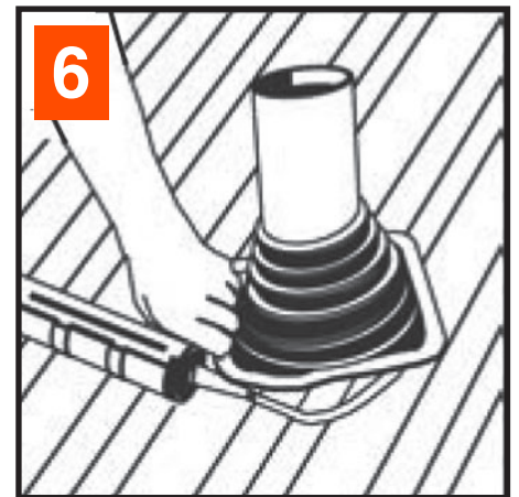
Apply sealant
