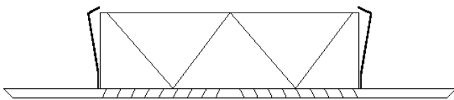
Speedi-GRILLE Clip-Design
