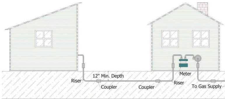
Figure 3.1 2 PSI Natural Gas Supply from House to Garage
