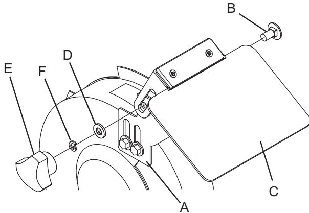
Figure 7 - Eyeshields
