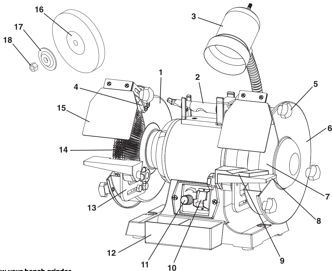
Figure 2 - Know your bench grinder.
