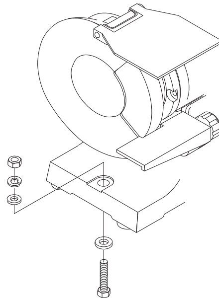
Figure 9 - Permanent Mounting
