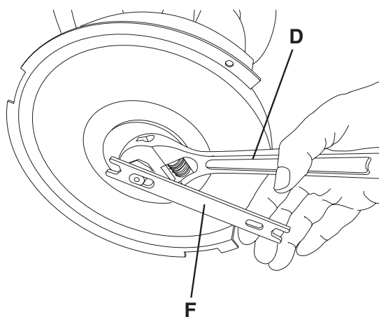
Figure 15 - Using wrenches to change the grinding wheel.
