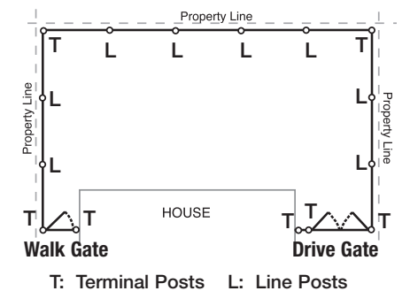
Sample Fence Layout
