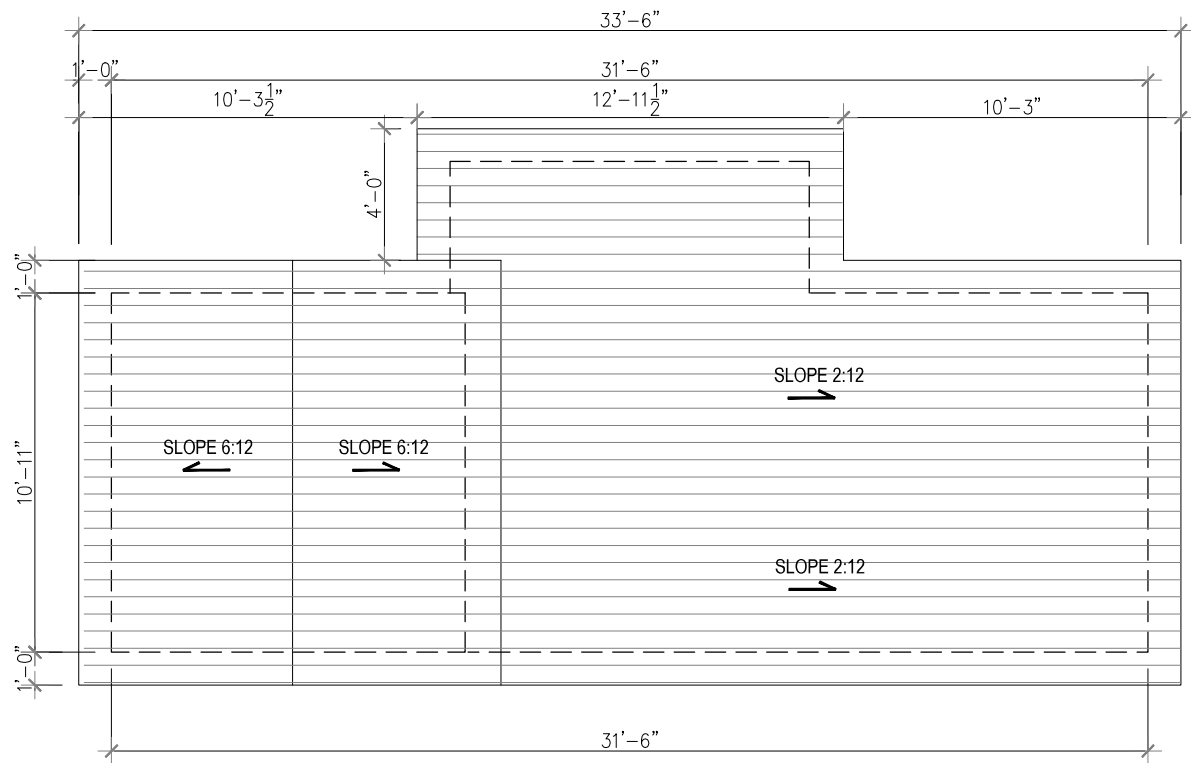
1 ROOF FLOOR PLAN Scale 1'=1/4"
