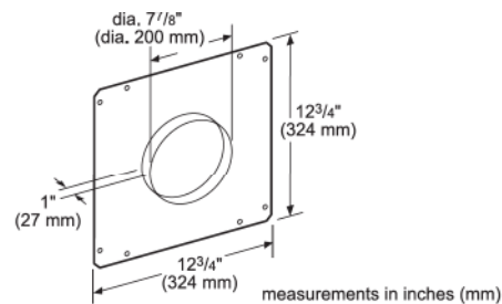
HDDFTRAN8 8" Round Front Plate for Downdraft
