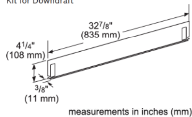
HDD6RSP 36" Gas Cooktop Seal Kit for Downdraft
