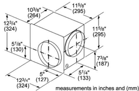
DHG602DUC 600 CFM Flexible Integral Blower – HDD Downdrafts
