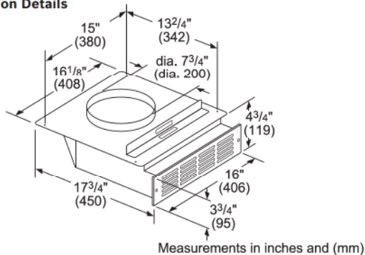
HDD6RSP 36" Gas Cooktop Seal Kit for Downdraft
