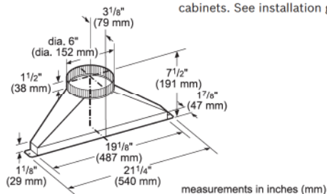
HDDSTRAN6 6" Side/Rear/ Downward Transition for Downdraft
