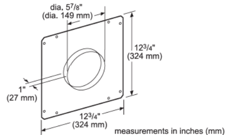
HDDFTRAN6 6" Round Front Plate for Downdraft
