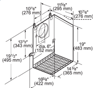
DHG6023RUC 600 CFM Remote Blower
