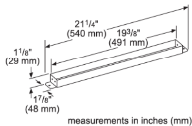
HDDSTRAN2 Transition for Rectangular Duct for Downdraft
