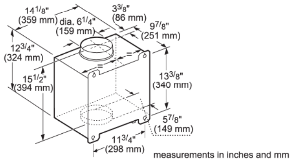
DHG6015NUC 600 CFM Inline Blower
