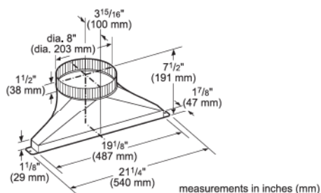
HDDSTRAN8 8" Side/Rear/ Downward Transition for Downdraft
