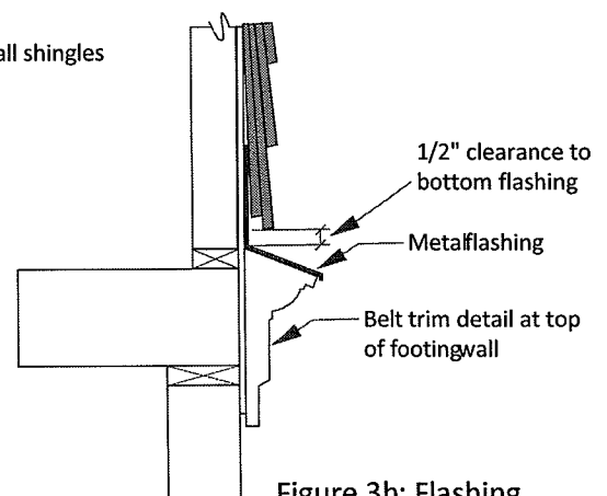
Figure 3b: Flashing
