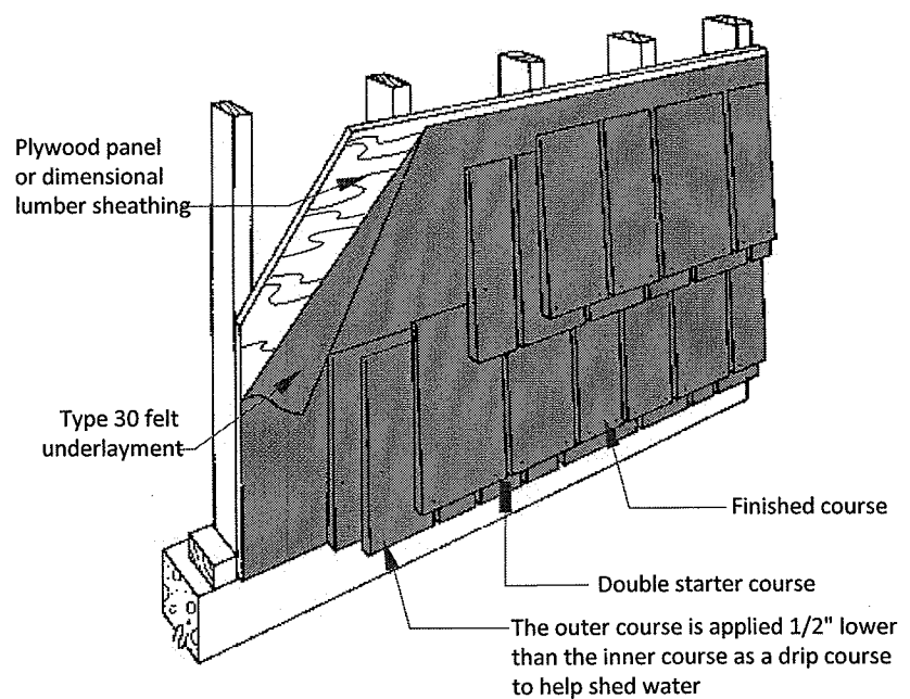
Figure 11: Ribbon Coursing
