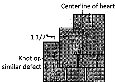
Figure 5: Course Alignment Nails
