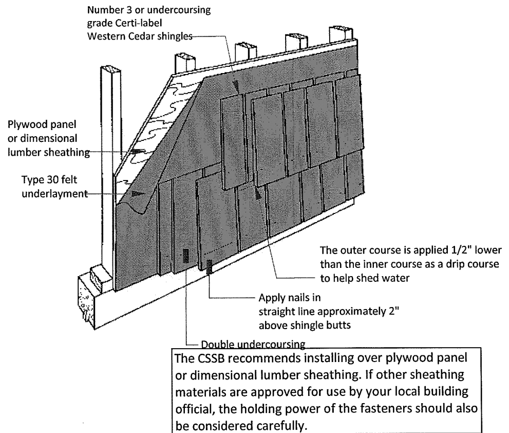
Figure 7: Double Coursing
