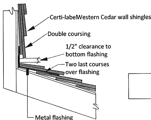
Figure 3a: Flashing
