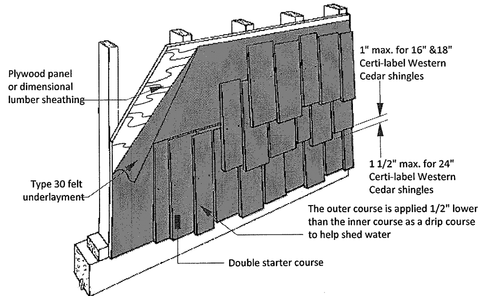
Figure 10: Staggered Coursing
