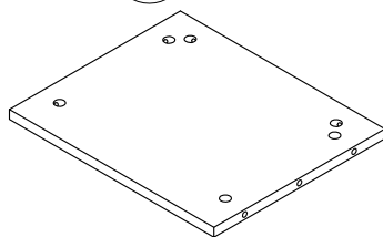
SIDE PANEL Panel lateral T9820096060 QTY:2
