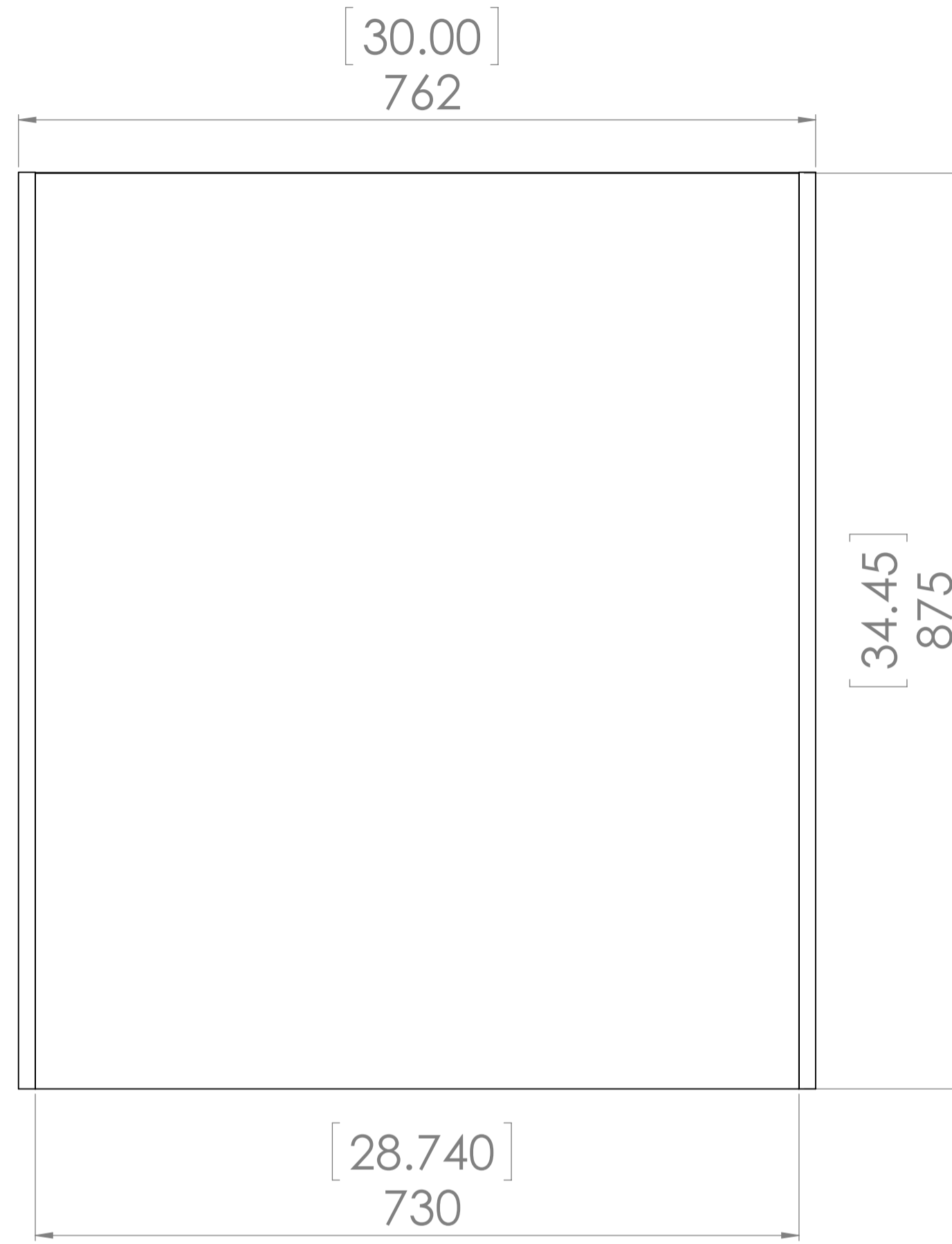
Back View
