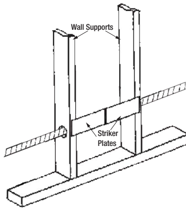
Figure 4.11b Shielding at Support Area and Between Wall Supports
