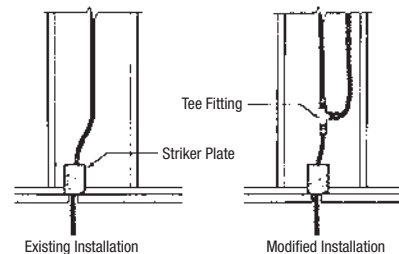
Figure 4.9 Extension of Existing Tubing Run
