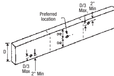
Figure 4.4 Holes in Wood Structures
