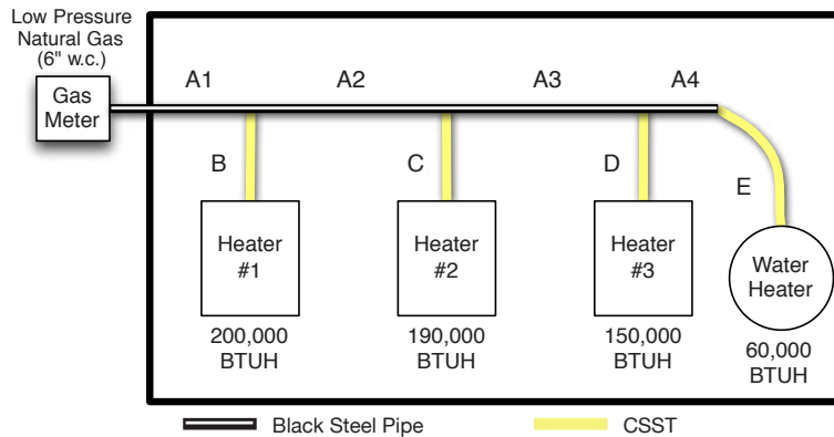
Figure 3.9 Low Pressure Hybrid System—Series Arrangement
