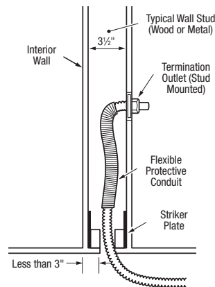
Figure 4.12 Use of Flexible Protective Conduit
