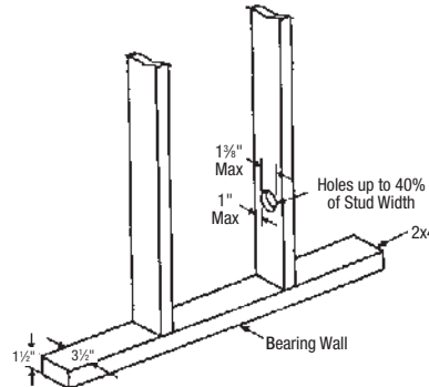
Figure 4.7 Holes in Bearing Walls
