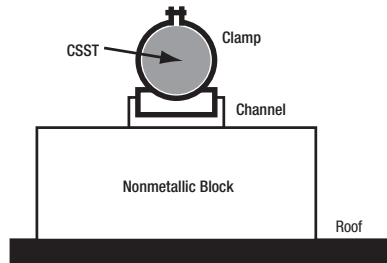
Figure 4.19 Rooftop Support with Strut
