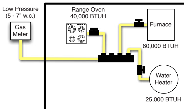
Figure 3.3 A low pressure parallel layout
