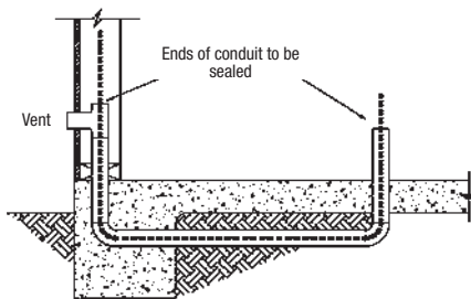
Figure 4.27 Installation in Nonmetallic Conduit with Venting
