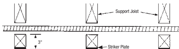
Figure 4.11a Shielding at Support Area When Penetration is 3 inches from edge
