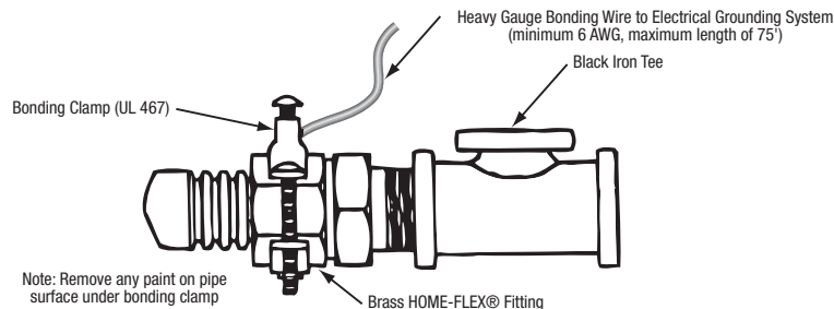
Figure 4.30 Bonding Connection to Brass Fitting
