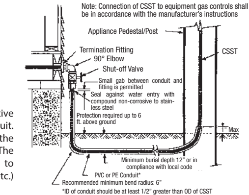
Figure 4.22 Fixed Outdoor Appliance (Underground Routing)
