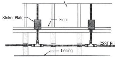
Figure 4.8 Multiple Outlets Along Main CSST Run
