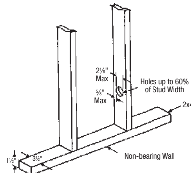
Figure 4.6 Holes in Non-Bearing Walls
