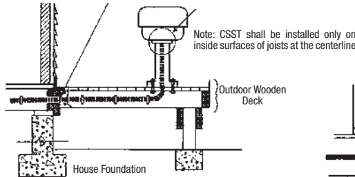
Figure 4.21 Fixed Outdoor Appliance (Deck Mounted)
