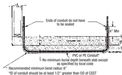
36 Figure 4.28 Installation in Nonmetallic Conduit Under Slab
