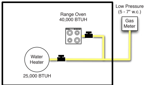
Figure 3.2 A low pressure series layout
