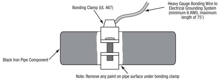
Figure 4.31 Bonding Connection to Rigid Black Iron Pipe
