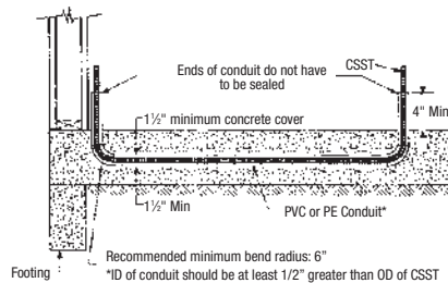
Figure 4.29 Installation in Nonmetallic Conduit In Slab
