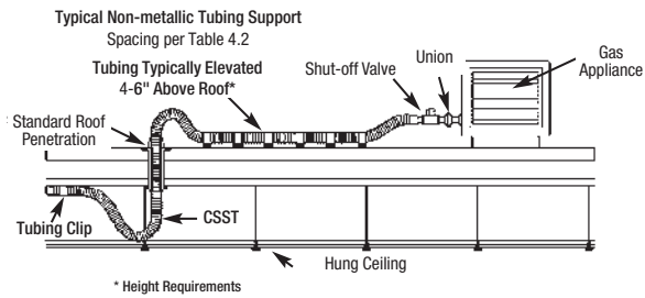
Figure 4.18 Roof Top Equipment Installation
