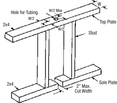
Figure 4.5 Holes and Cuts in Top and Sole Plates
