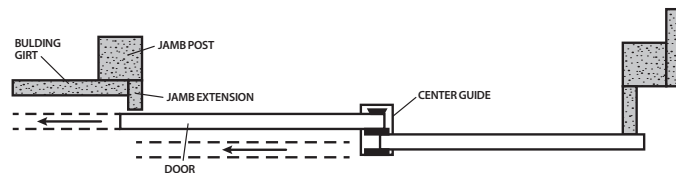
2 - DOOR TOP VIEW (TYPICAL)
