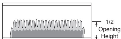
Figure 26 - Correct Burner Flame Pattern
