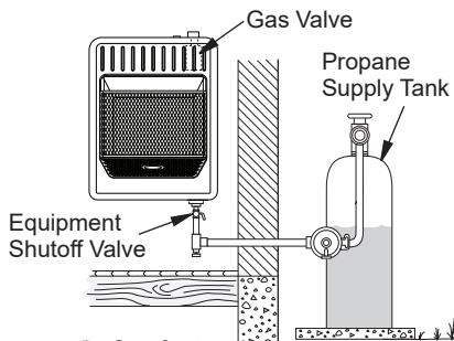
Figure 19 - Checking Gas Joints for Propane Gas
