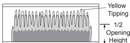
Figure 27 - Incorrect Burner Flame Pattern
