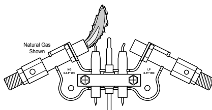
Figure 25 - Incorrect Pilot Flame Pattern
