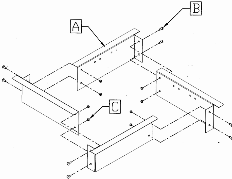
ASSEMBLY OF SQUARE FIRERING INSERT
