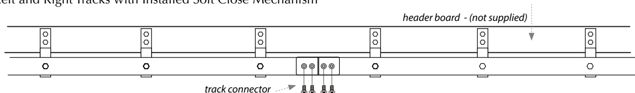
Left and Right Tracks attached to header board with installed track connectors
