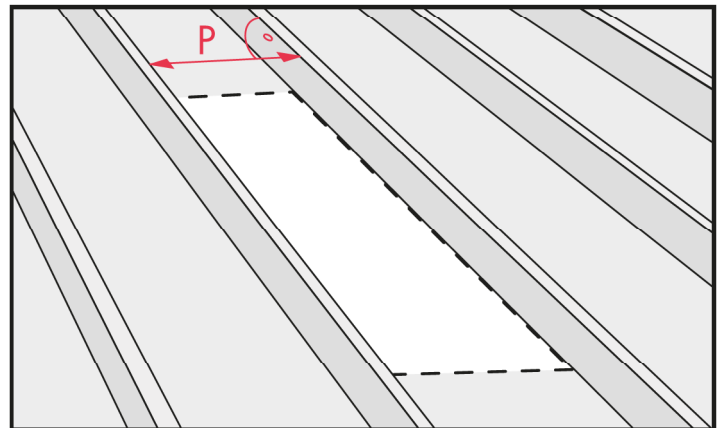
Fig.12. P- Distance between the ceiling joists.
