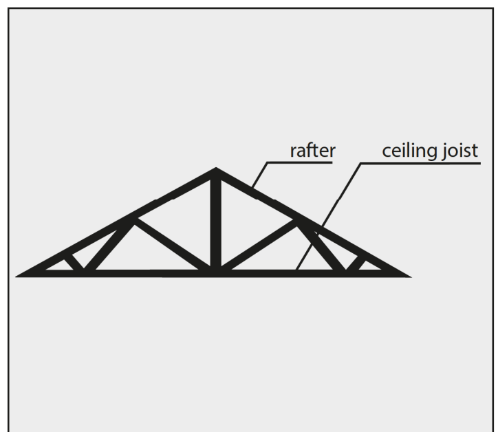
Fig.3. Truss roof frame.
