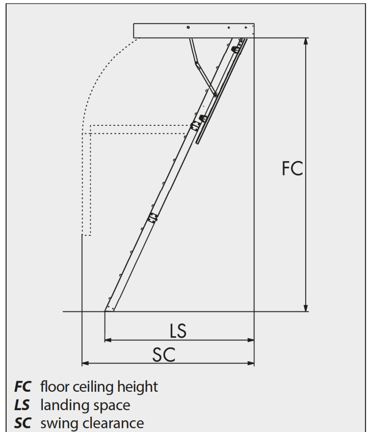
Fig.4. Characteristics of the attic ladder.
