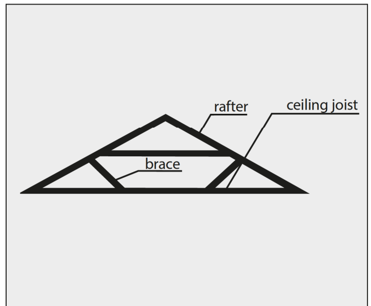
Fig.2. Typical construction of the roof with braces connected to the ceiling joists.
