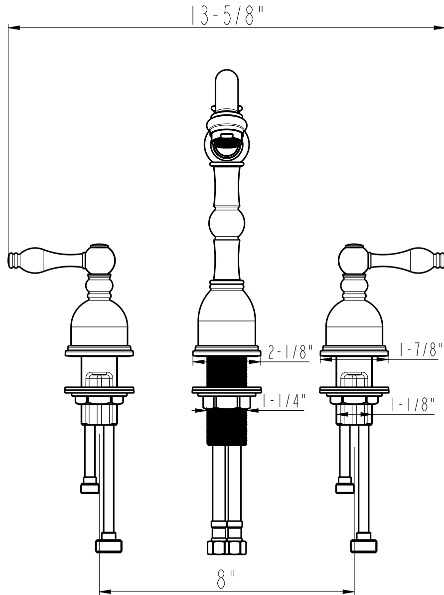
41518-Dimensional drawing
