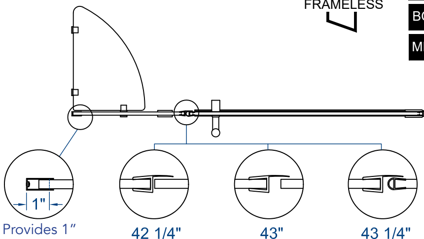
DOOR GAP AT DIFFERENT OPENING WIDTHS
