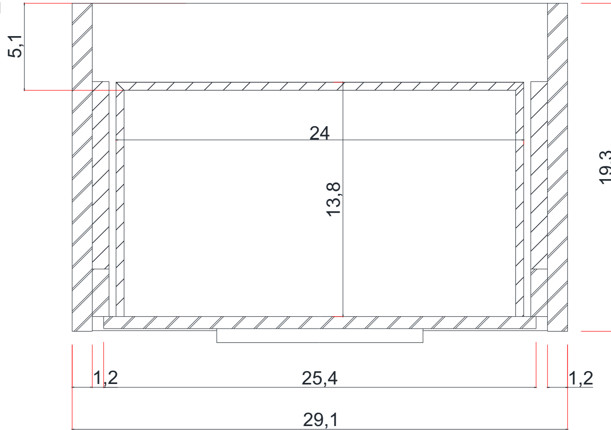
TOP WIEV C-C SECTION
