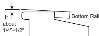
Wooden Window
