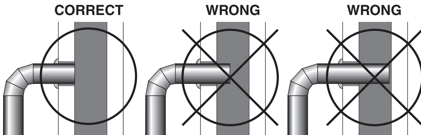
Fig. 10 – Stovepipe/Flue Connections
