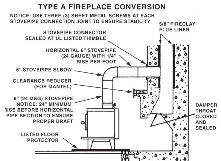
Fig. 14 - Fireplace Conversion
