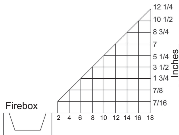
Fig. 3 - Minimum Clearance for Combustible to Wall
