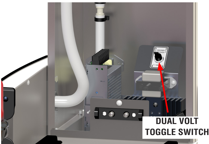
120/208-240V 3 WIRE + GROUND
