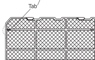
Air Filter
