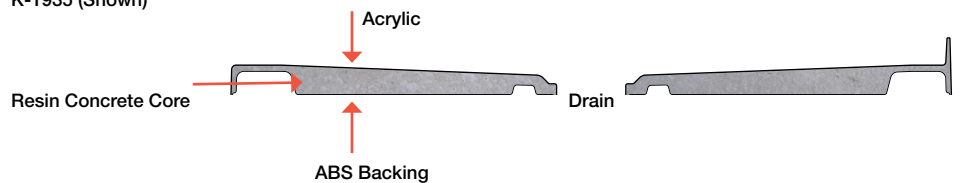
Cross section for Ballast® shower base K-1935 (Shown)
